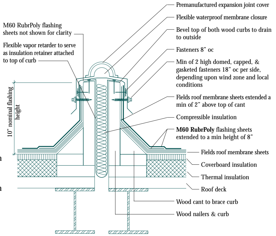
Side View
