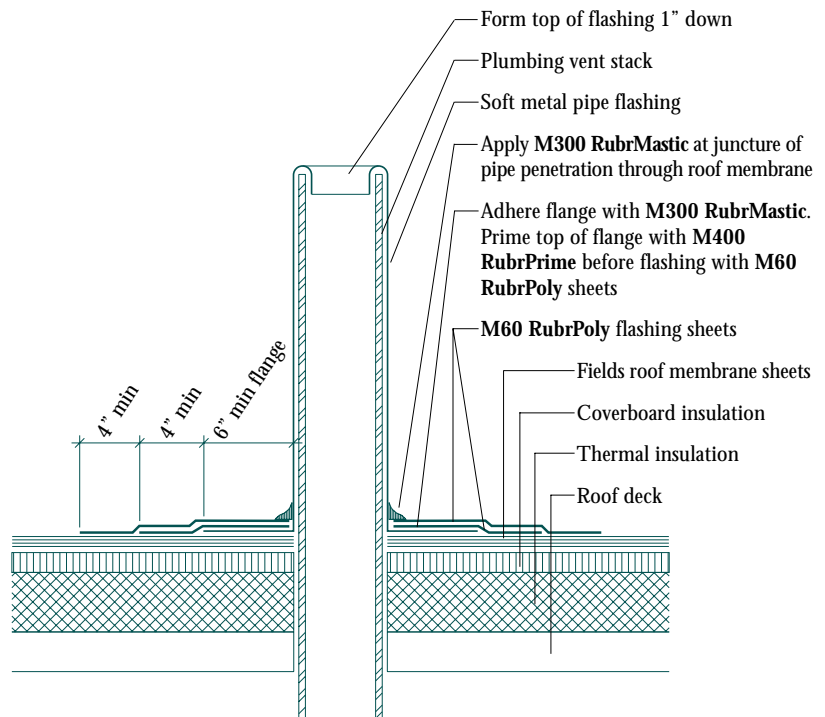
Side View
